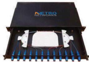
12F Loaded Rackmount LIU
