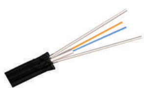
2 Core 2 FRP Cable, G652D Diameter 5.8, HDPE
